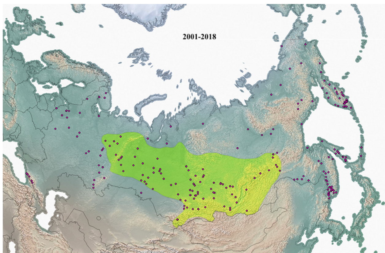
Figure 3 Spatial distribution of brown bear attacks during 2001–2018 within (yellow-green color) and outside the Siberian pine ( Pinus sibirica ) range in Russia (Malyshev et al. 2008).
