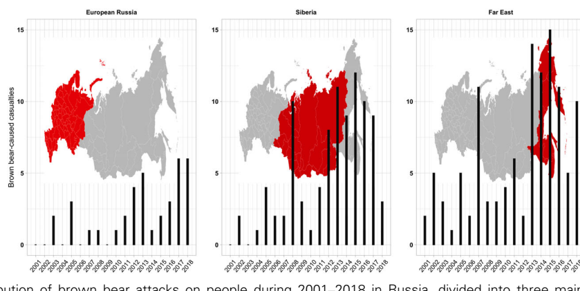
Figure 2 Spatial distribution of brown bear attacks on people during 2001–2018 in Russia, divided into three main geographical regions – European Russia [4 350 626 km 2 ; brown bear population ~ 72 165 (2018)], Siberia [9 917 620 km 2 ; brown bear population ~ 91 700 (2018)], and the Far East [3 112 700 km 2 ; brown bear population ~ 63 000 (2018)].
